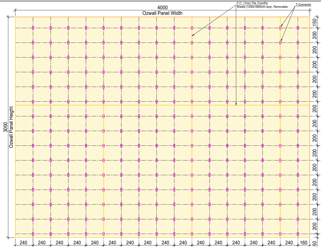
ELEVATION - B [ACCESSIBLE SIDE] F17, 17mm thk Formply Sheet (1200x1800 sheet size) & T-Connectors System for 4.0M x 3.0M Wall panel
