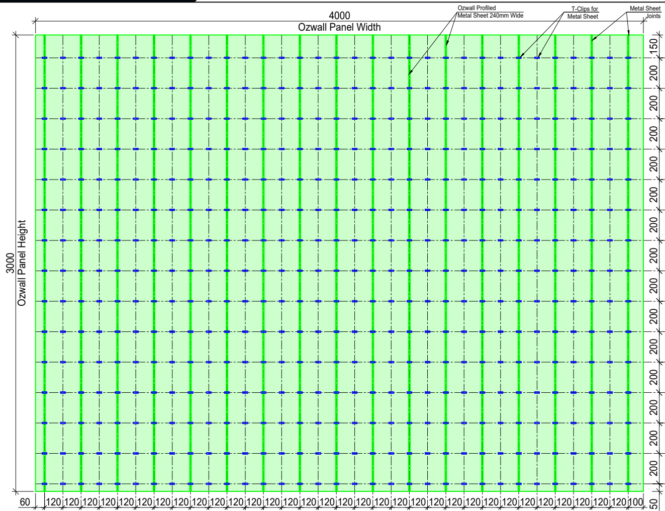
ELEVATION - A [IN-ACCESSIBLE SIDE] Ozwall Profiled Metal Sheet (Sacrificial) & T-Clips System for 4.0M x 3.0M Wall panel
